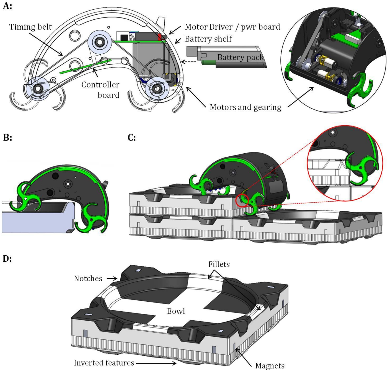
Figure 4.2.d. A: Cross section of the robot showing the drive system, controller and power electronics, the battery pack and the shelf it rests on. B: The raised center of the robot chassis helps it clear the corner of a brick as it climbs from the ground. C: Robot climbing up bricks, using hooks on the rear wheels for added traction. D: Brick showing features related to climbing and attachment.
