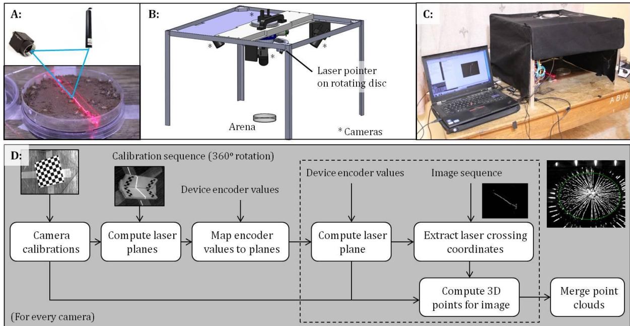
Figure 5.5.b. Laser scanner for continuous monitoring of termite construction in confined arenas. A: shows the geometric concept with a line laser and a camera. B: shows a simulated view of the device developed. C: Photo of the real device in Namibia 2012. D: Process by which the data from the device and images from the cameras on it are transformed into 3D height maps.
