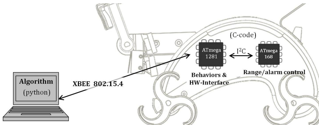
Figure 4.6.f. Processors involved in the control of a TERMES robot. The algorithmic layer of the software is implemented on a laptop, the main processor runs the behavioral- and hardware layers. A separate processor handles all code related to both ranging and alarm signals.
