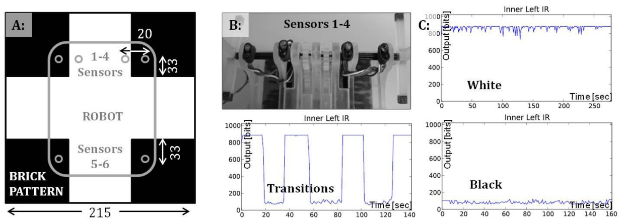
Figure 4.3.a. Brick patterns and IR transceivers. A: Dimensions of grid pattern and position of \sensors, top view, all dimensions are in mm. B: Configuration of transceivers in CliRob. C: Example of output from a sensor as the robot drives over black and white surfaces.
