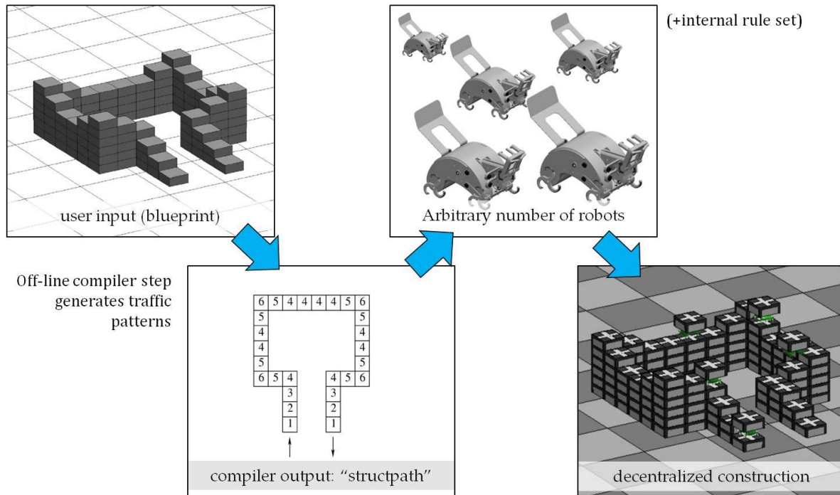
Figure 3.2.a. Overview of algorithmic framework.
