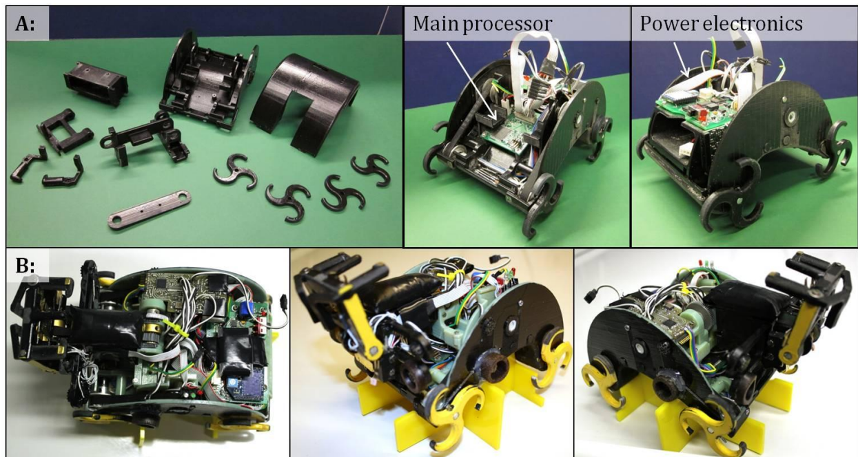
Figure 4.7.a. A: Assembly of Khali 2011. B: Isis 2013, showing wires between PCBs in the robot.
