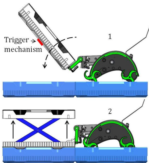
Figure 4.9.a. Bricks which automatically expand when placed to form columns, roofs, or bridges.
