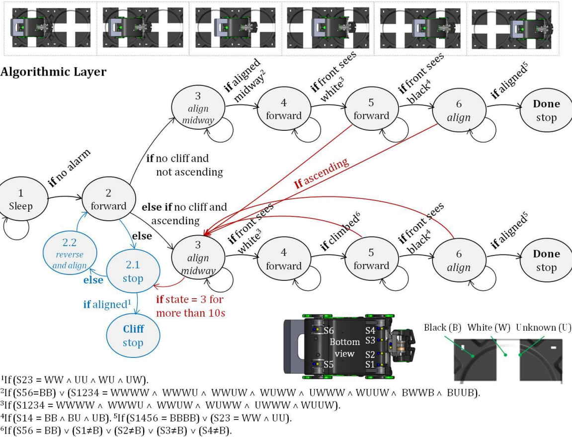
Figure 4.6.h. Block diagram for the routine to move forward one brick: “Go straight”. If-statements in the block diagram are clarified by footnotes and illustrations below.
