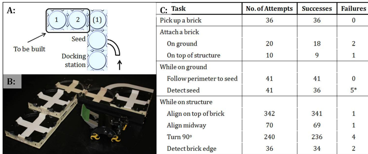
Figure 4.8.e. Consistency test with one robot building a 3-brick staircase 10 times a row. A: Schematic of the structure to be built in extension of the seed brick, the docking station and a fixed brick (1). B: Photo of completed structure. C: Successes (including error recovery) and failures of sub-tasks in the experiment. The total process took about 4hrs; the battery was replaced twice.
