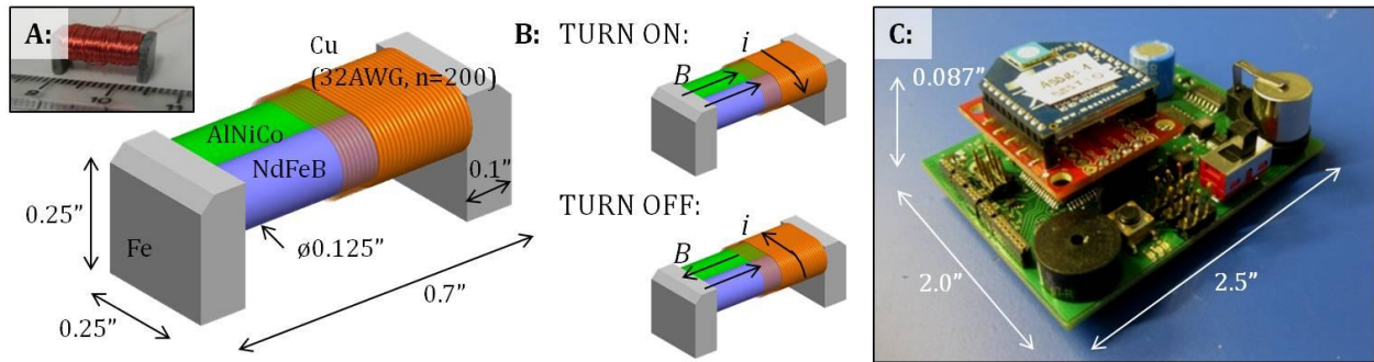
Figure 4.9.b. Smart brick components. A: Design of electro-permanent magnet (EPM) with a holding force of 318g when attached to a 10mm thick iron rod. B: How to turn the EPM on and off. C: Circuitry developed to fit in a smart brick with the ability to control up to 8 EPMS.
