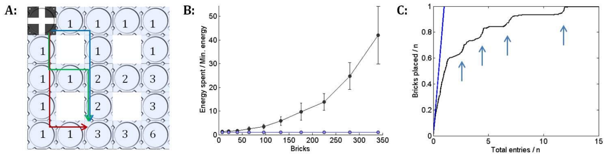
Figure 3.3.d. System performance for structures with paths that branch and join, see Figure 3.3.b.c. A: Shows how some places in the structure are more likely to be reached than others if the probability for choosing any branch is constant throughout the structure. The number in each square denotes the number of paths lead to it. B: Shows how performance scales with the number of bricks up to 341 (=100 squares). The energy spent is normalized with respect to the performance of a centralized controller, i.e. the minimum energy needed to complete the structure (also shown in blue). 100 replicas were done for each structure size. C: Example of structure progress over the number of agents which have entered the structure, normalized to the total number of bricks. The performance of the centralized system is shown in blue. The arrows indicate sudden bursts of activity in construction caused by depositions made to branching points on the edge of the structure; otherwise progress is slowed down because of the row rule.
