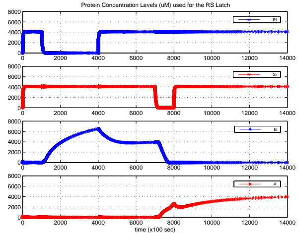
Figure 2: Dynamic Behavior of a Biological \overline{R}\overline{S} Latch
